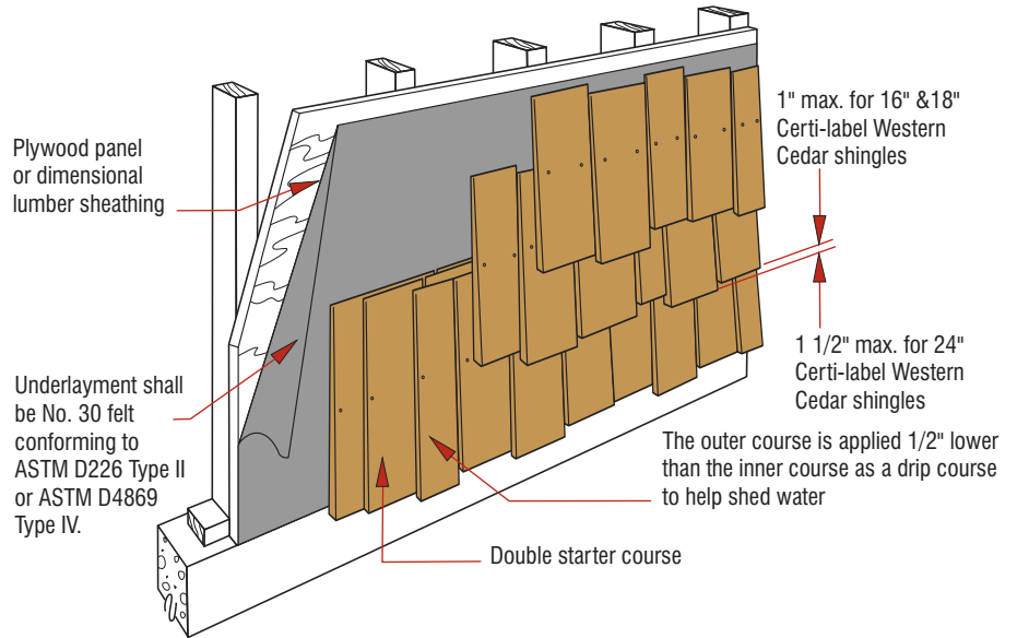
Figure 10: Staggered Coursing
